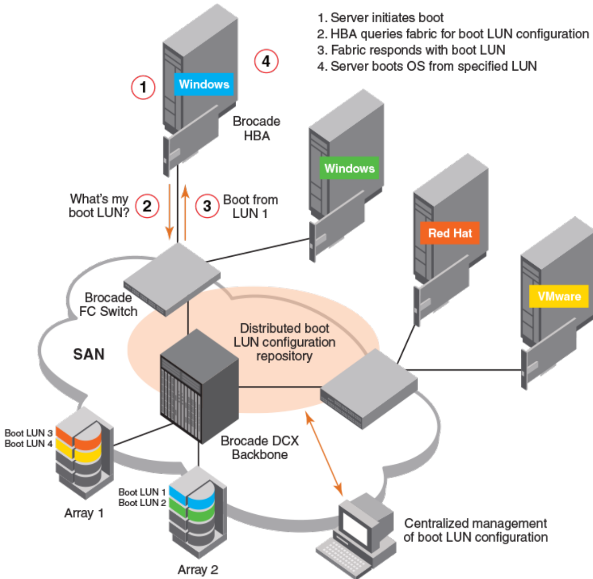
FIGURE 35 Boot LUN zoning
