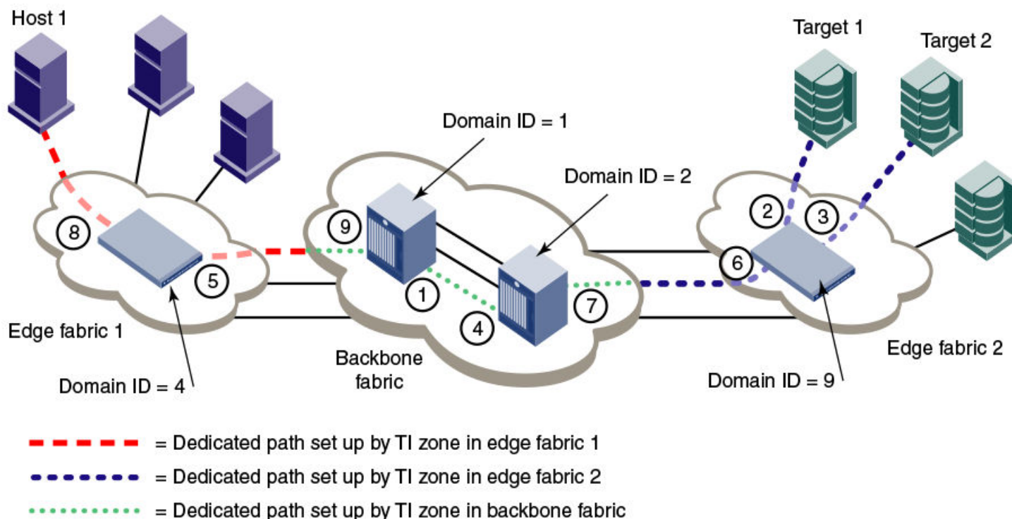
FIGURE 48 TI over FCR example
