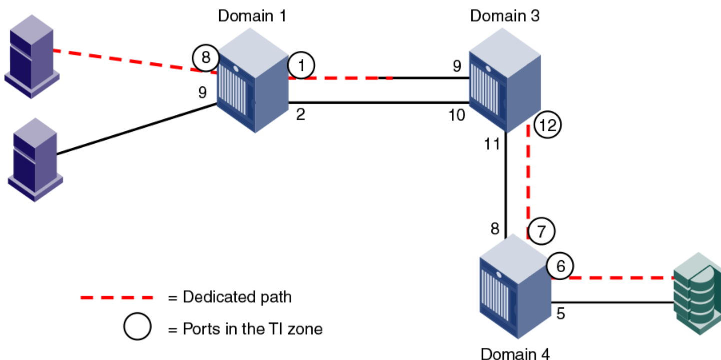
FIGURE 43 TI zone misconfiguration
