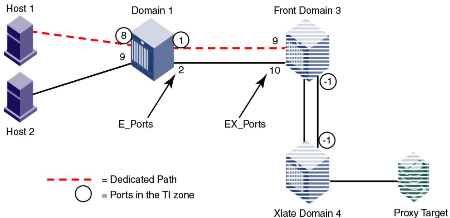
FIGURE 45 TI zone in an edge fabric
