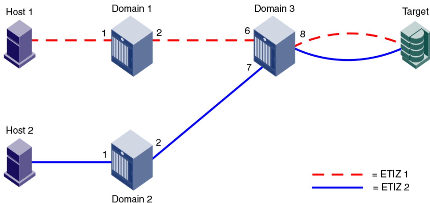
FIGURE 40 Enhanced TI zones
