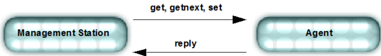
FIGURE 11 SNMP query
