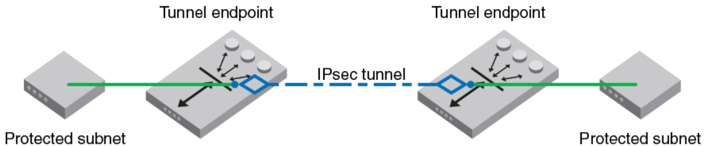
FIGURE 15 Gateway tunnel configuration
