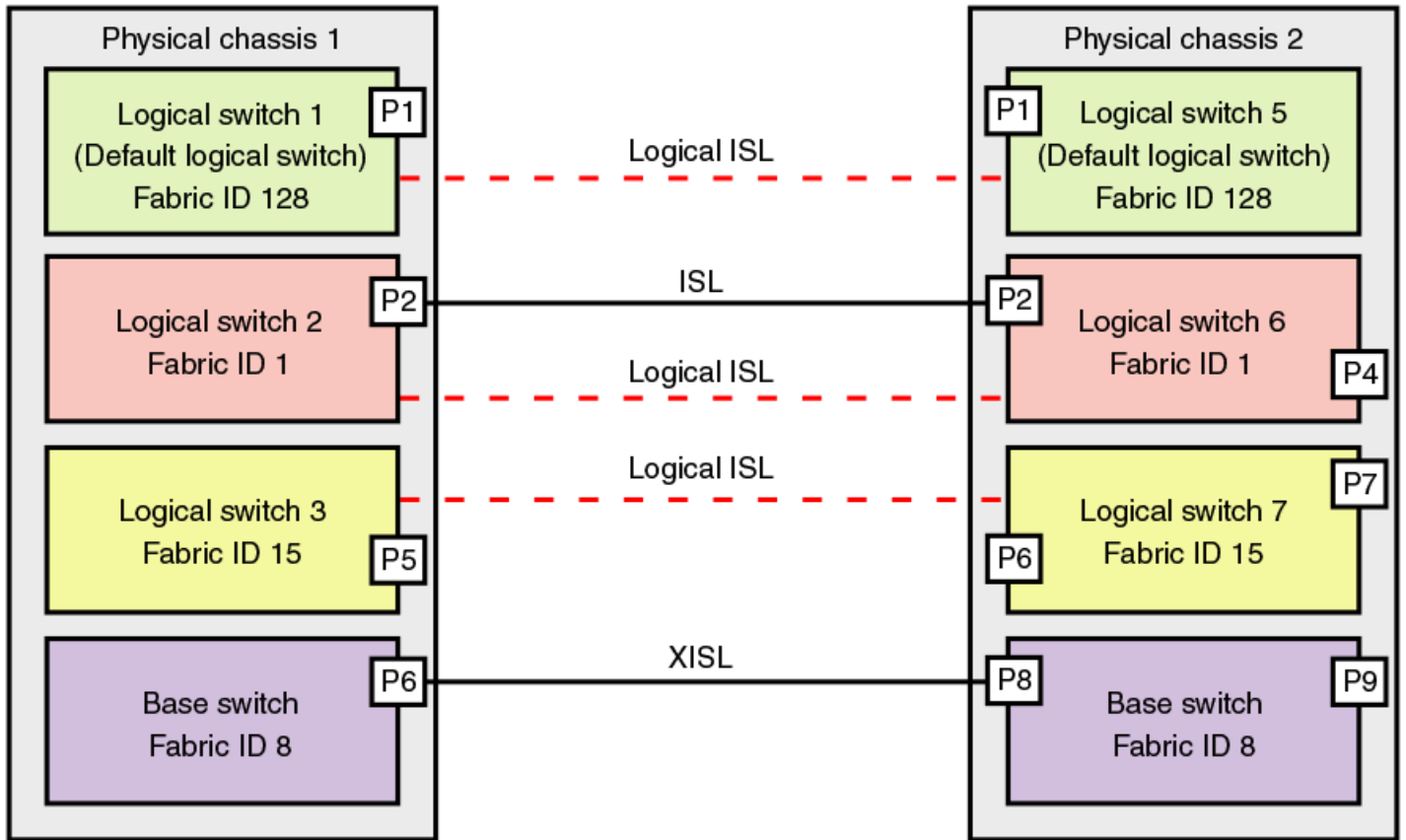
FIGURE 27 Logical fabric using ISLs and XISLs
