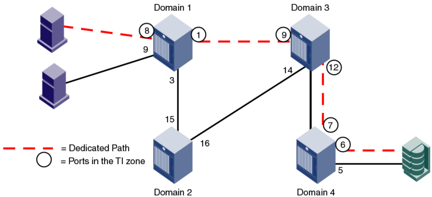
FIGURE 38 Dedicated path is the only shortest path
