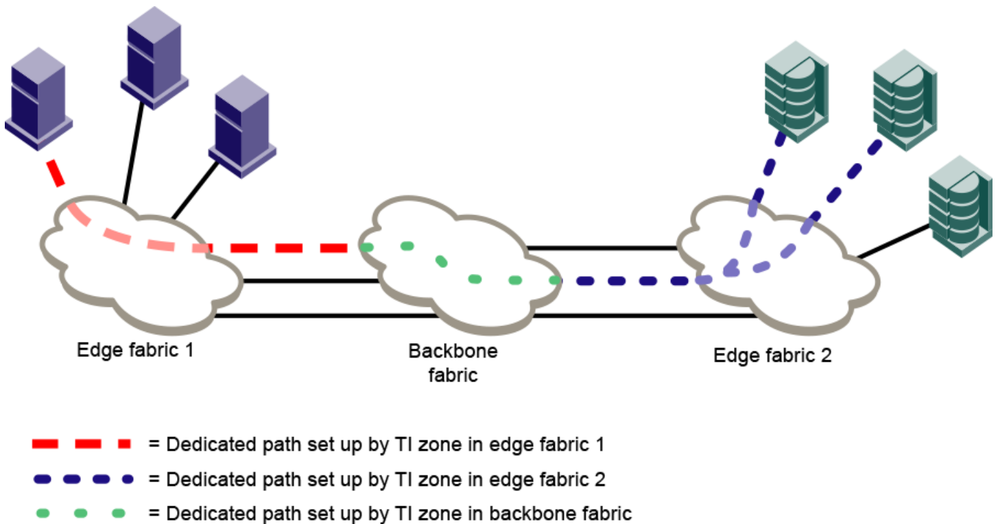
FIGURE 44 Traffic Isolation Zoning over FCR
