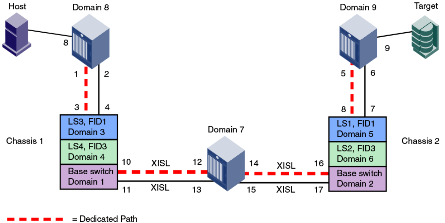
FIGURE 49 Dedicated path with Virtual Fabrics
