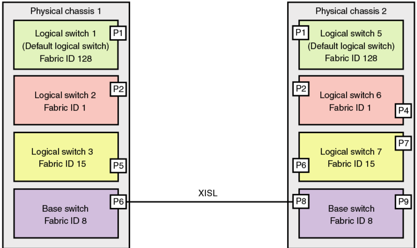
FIGURE 25 Base switches connected by an XISL
