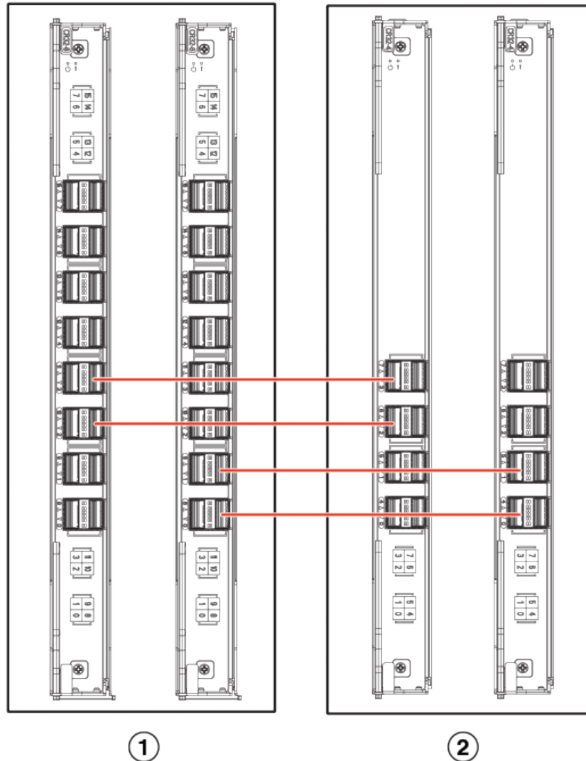
FIGURE 67 Minimum configuration for 128 Gbps ICLs
