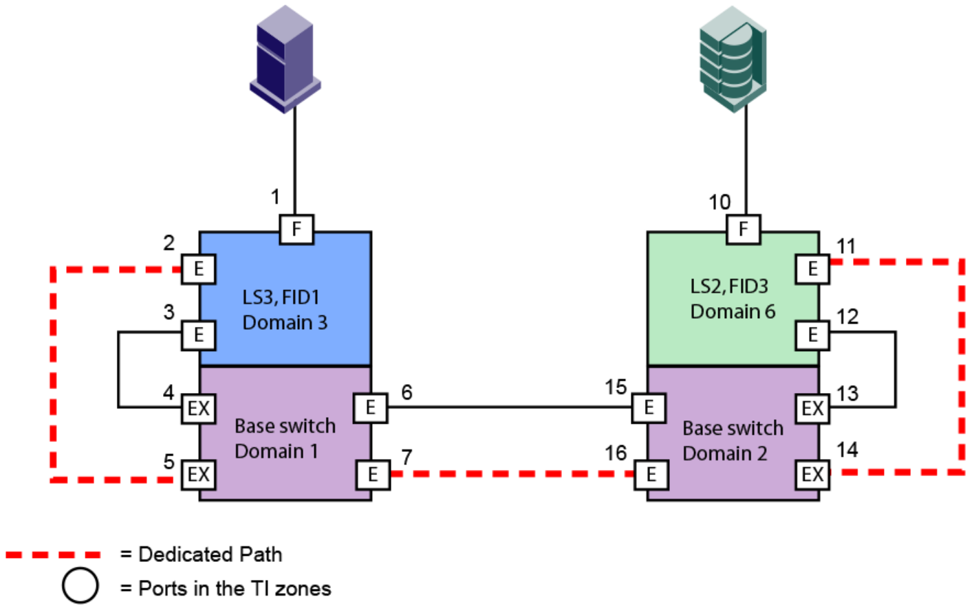
FIGURE 52 Example configuration for TI zones over FC routers in logical fabrics
