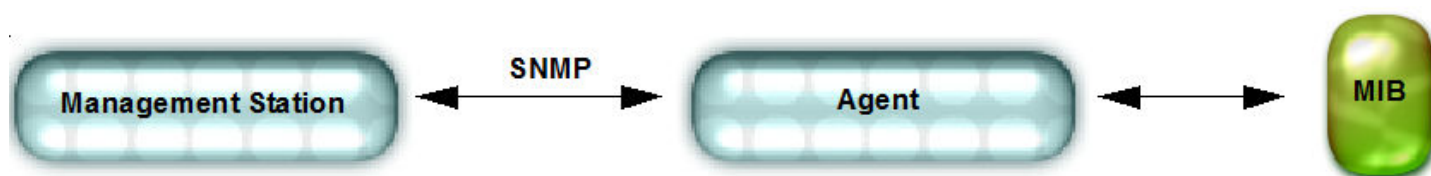
FIGURE 10 SNMP structure
