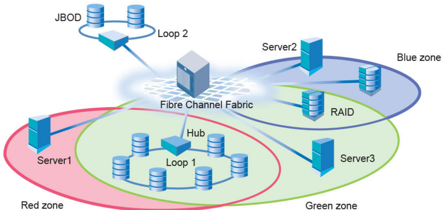
FIGURE 29 Zoning example
