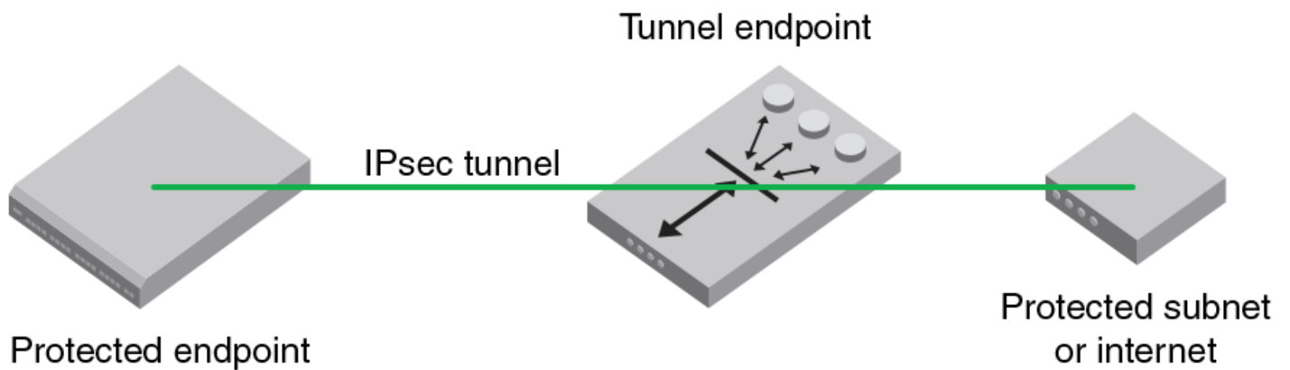
FIGURE 16 Endpoint-to-gateway tunnel configuration
