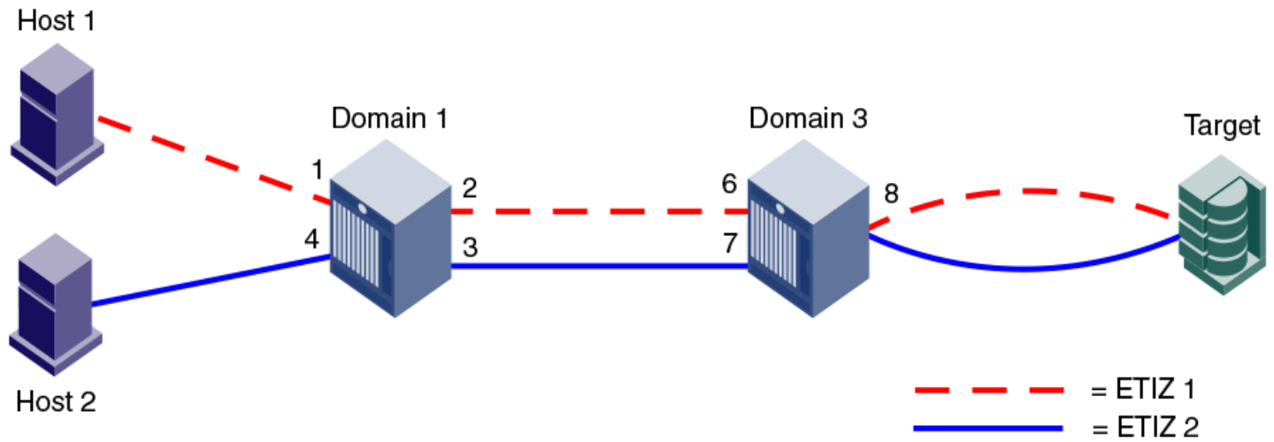
FIGURE 41 Invalid ETIZ configuration: two paths from one port to two devices on the same remote domain
