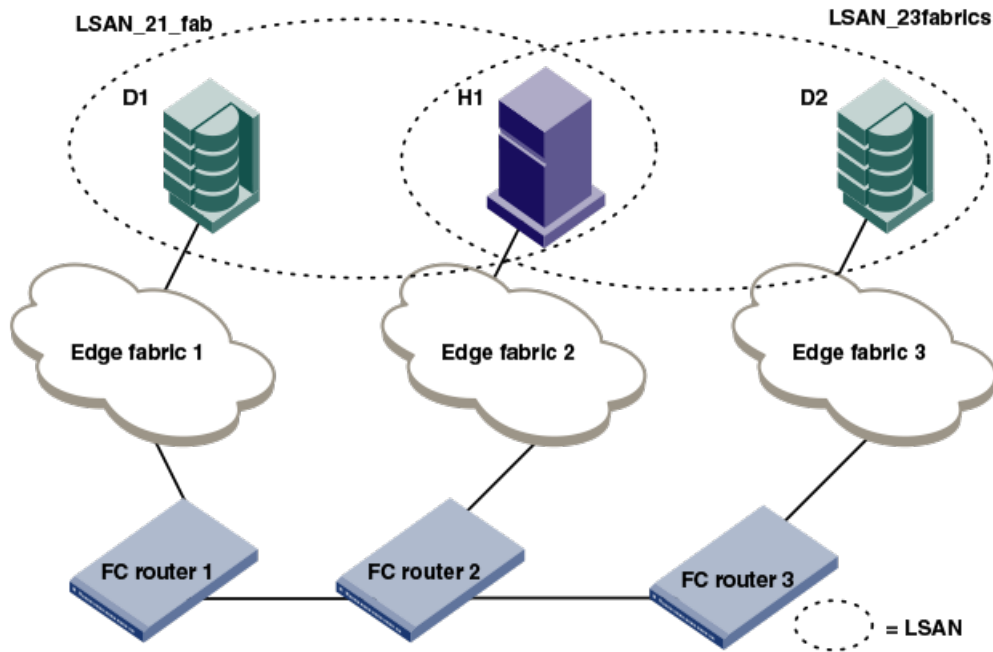
FIGURE 82 Example of setting up Enforce LSAN tag
