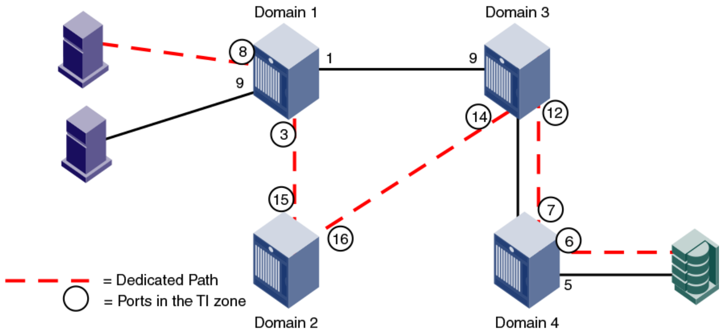
FIGURE 39 Dedicated path is not the shortest path
