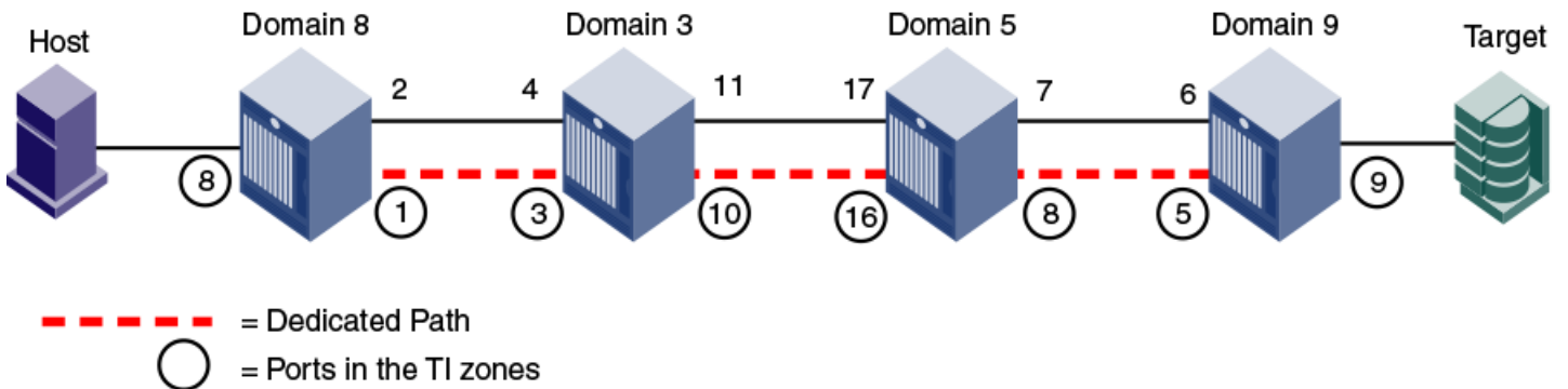
FIGURE 50 Creating a TI zone in a logical fabric
