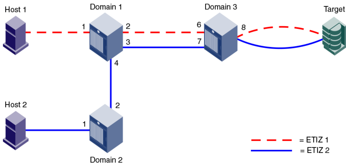
FIGURE 42 Invalid ETIZ configuration: two paths from one port
