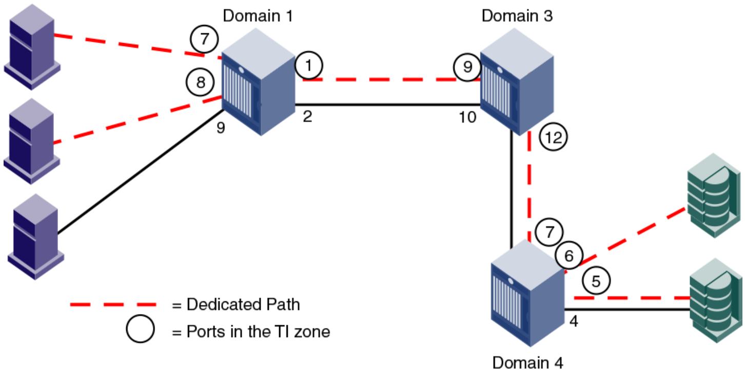
FIGURE 37 Traffic Isolation zone creating a dedicated path through the fabric
