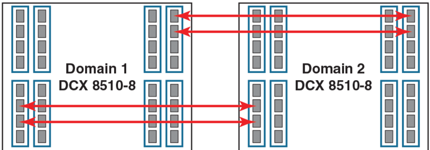
FIGURE 66 Minimum configuration for 64 Gbps ICLs
