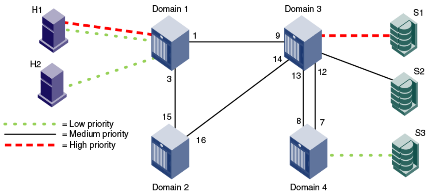
FIGURE 56 QoS traffic prioritization
