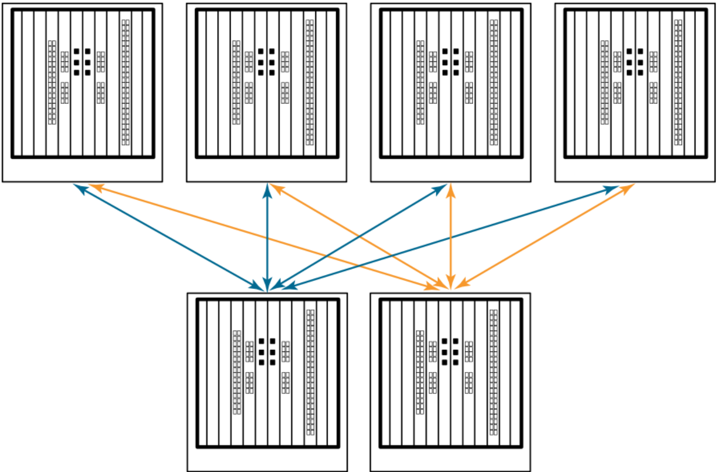
FIGURE 71 Gen 5 DCX 8510 64 Gbps ICL core-edge topology
