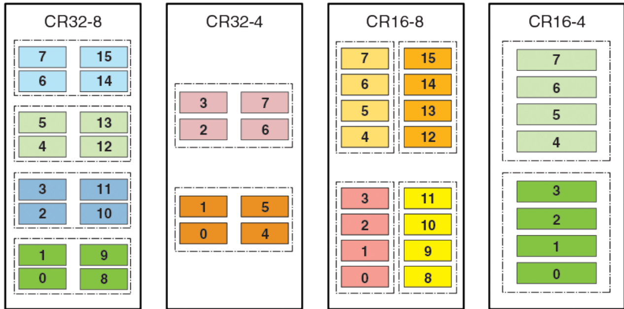
FIGURE 68 Port groups in Gen 5 CR blades vs Gen 6 CR blades
