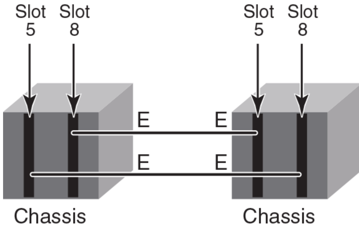
FIGURE 60 ICLs connecting chassis blades
