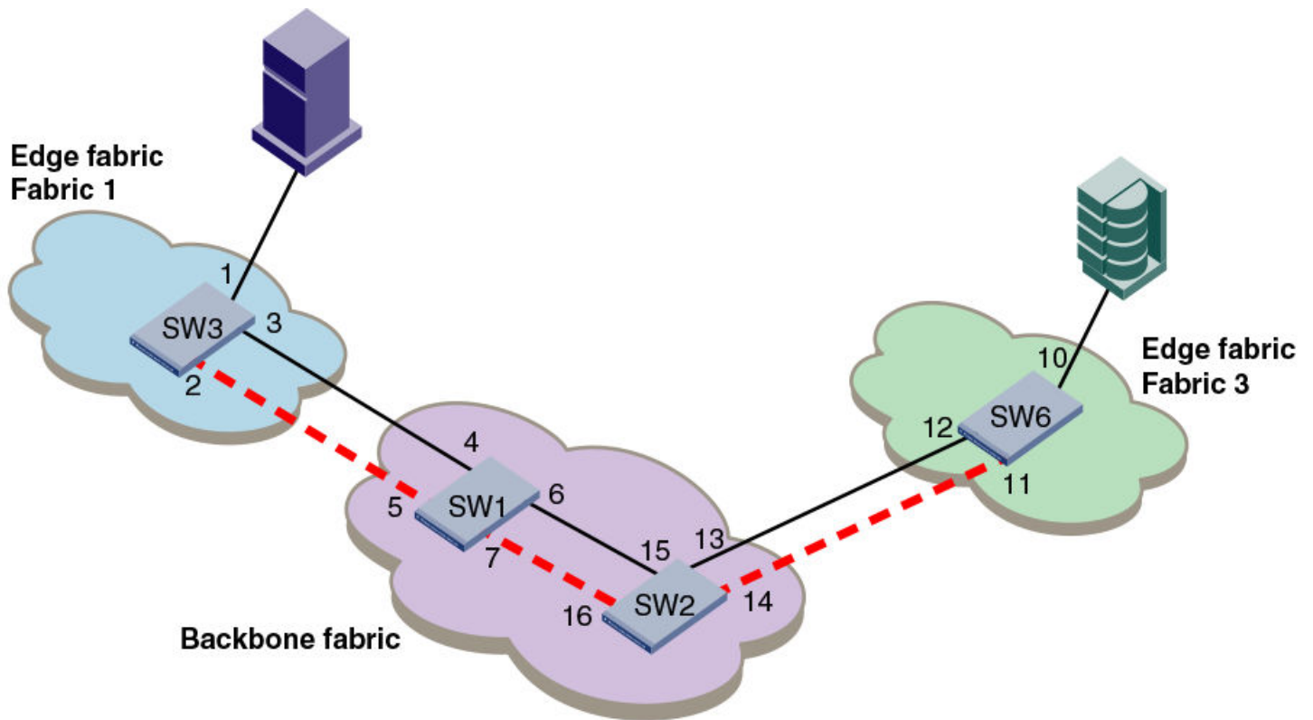
FIGURE 53 Logical representation of TI zones over FC routers in logical fabrics
