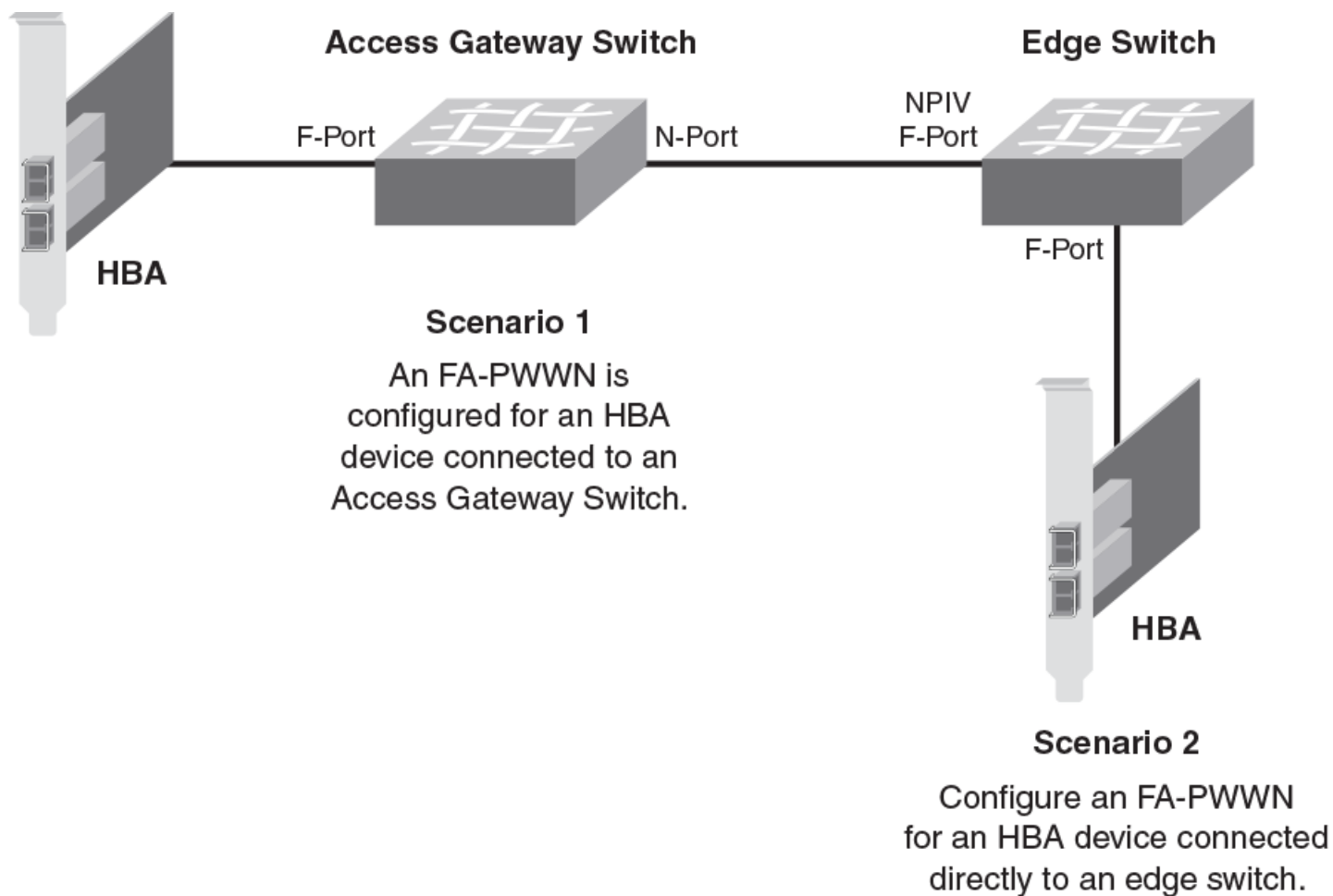
FIGURE 65 Fabric-assigned port World Wide Name provisioning scenarios
