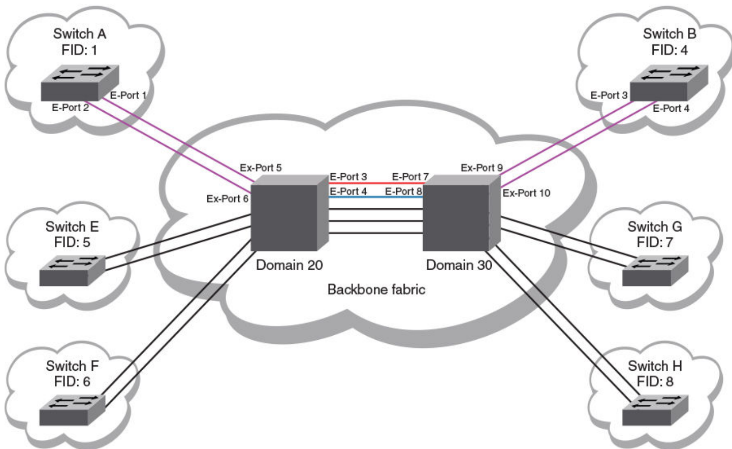
FIGURE 47 Fabric-level traffic isolation
